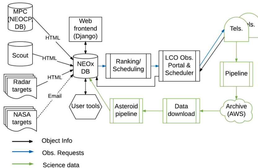
Fig. 2. Schematic overview of the NEOexchange TOM system. Targets for follow-up are ingested into the NEOx DB (center) from the data source (left side), planned and scheduled and sent to follow-up telescopes (right). The resulting data flows through the observatory data reduction pipeline and into the archive. This is retrieved by NEOexchange and processed through science specific pipelines and the results of these are also stored in the NEOx DB.
